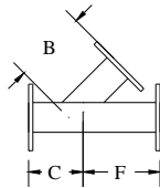
45° LATERAL PLAIN END OR FLANGED
