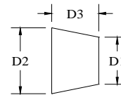
CONCENTRIC REDUCER PLAIN END OR FLANGED
